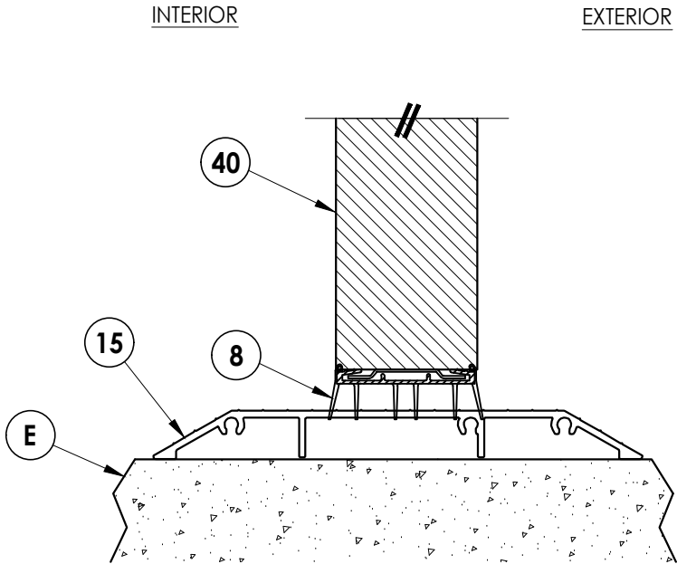
3 3 VERTICAL CROSS SECTION Inswing Shown
