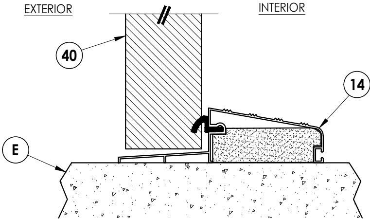
2 3 VERTICAL CROSS SECTION Outswing Shown
